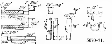
Figs. 5067-69. BRAKE-LEVER SPRING AND EYE-GUIDES.
